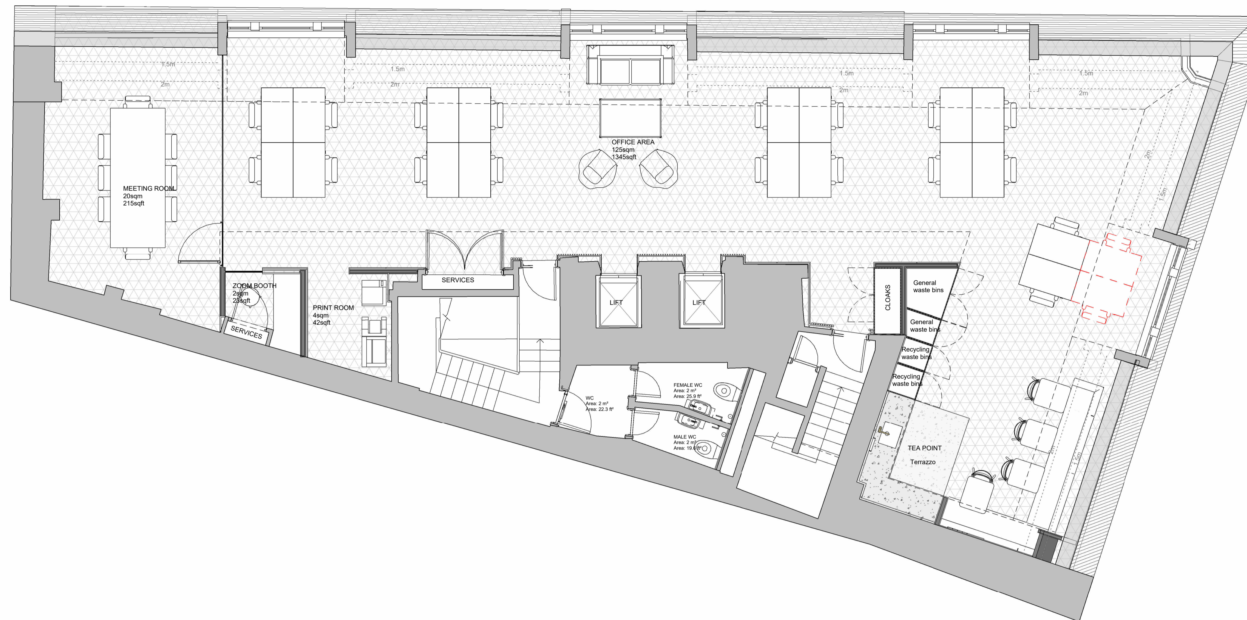
1 Proposed Fifth Floor - Furniture Plan 1 : 50
